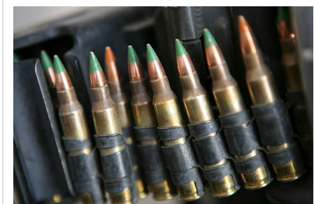
M855 and M856 cartridges in an ammunition belt using M27 disintegrating links.
